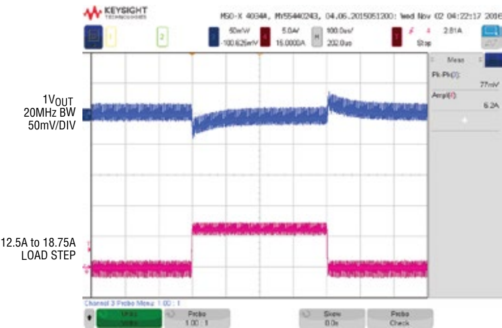
Figure 4. Measured Channel 1, 12.5A to 18.75A Load Transient ( V_{IN} = 12V , V_{OUT1} = 1.0V )
